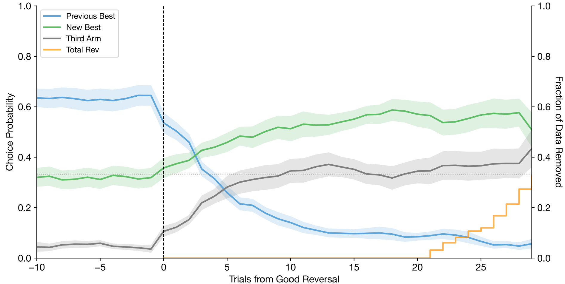
Reversal-Aligned Choices (mean \pm se across problems | n=6 subjects, n=132 reversals, n=17 problems)
